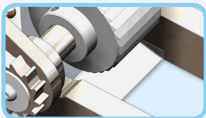
Large blade for up to 60mm bead width.
